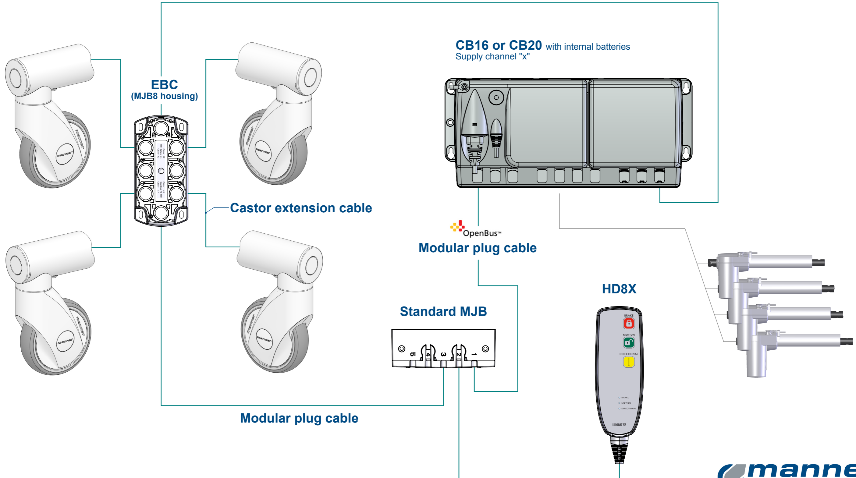
Cable between CB16/CB20 & EBC
